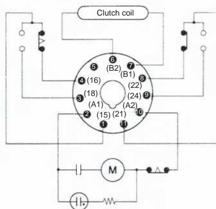
H2C(-F)R/H2C-SR
