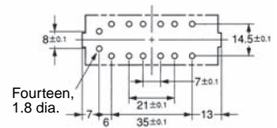
Mounting Hole Dimensions
