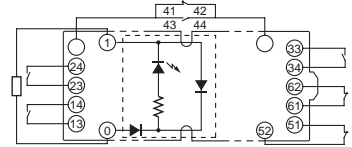
Terminal Arrangement/Internal Connection Diagram (Top View)
