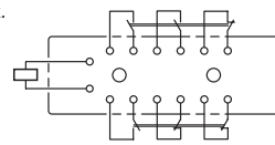
With G7S-3A3B mounted
