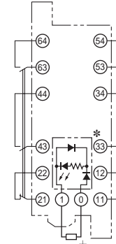
G7SA-4A2B Mounted
