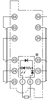
G7SA-5A1B Mounted
