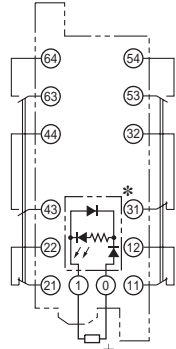
G7SA-3A3B Mounted
