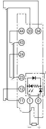
G7SA-3A1B Mounted
