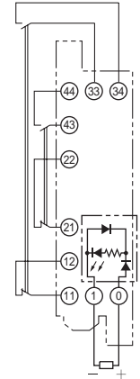
G7SA-2A2B Mounted
