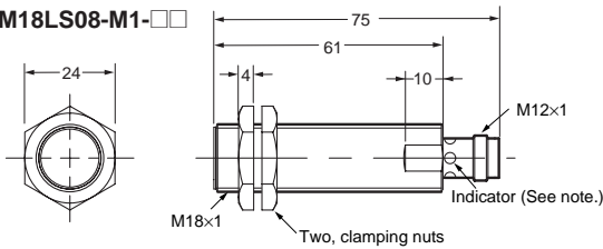
E2A-M18LS08-M1-□□
