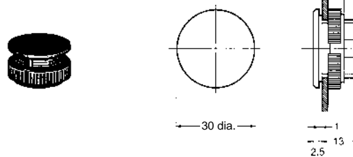
For Projection Models A22Z-3600T
