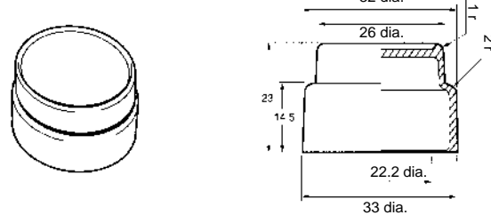
For Projection Models A22Z-3600T
