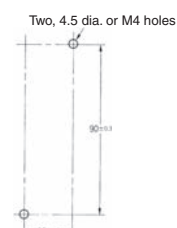
Mounting Holes
